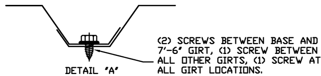
"A" PANEL - WALL
